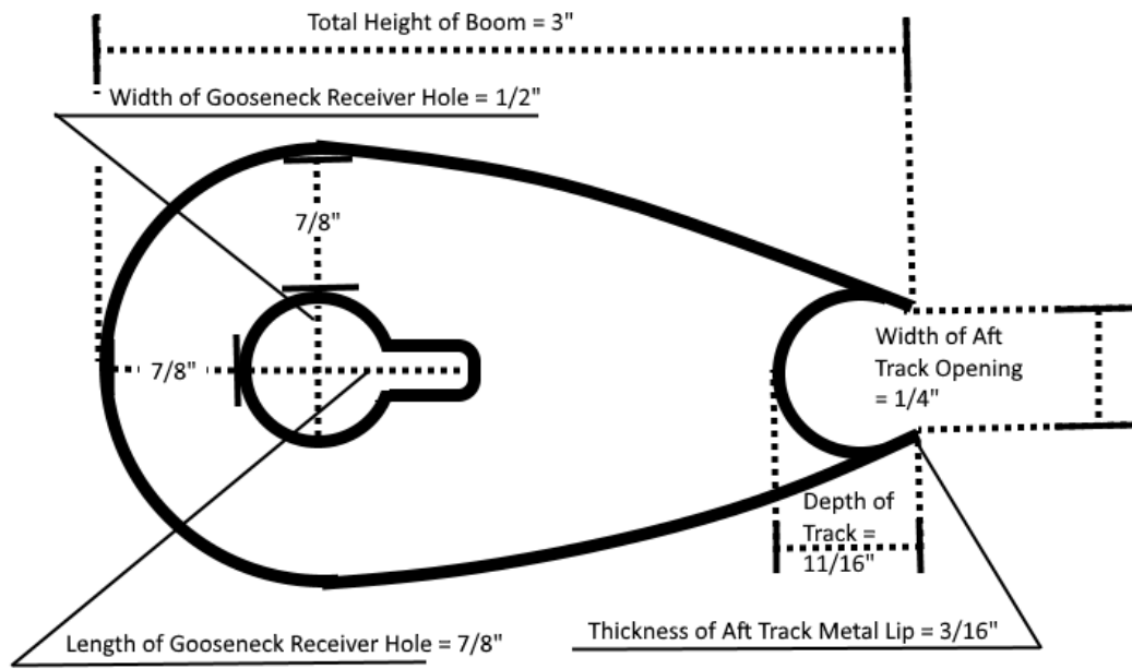
FIGURE 4: Boom Profile Fore Edge View
